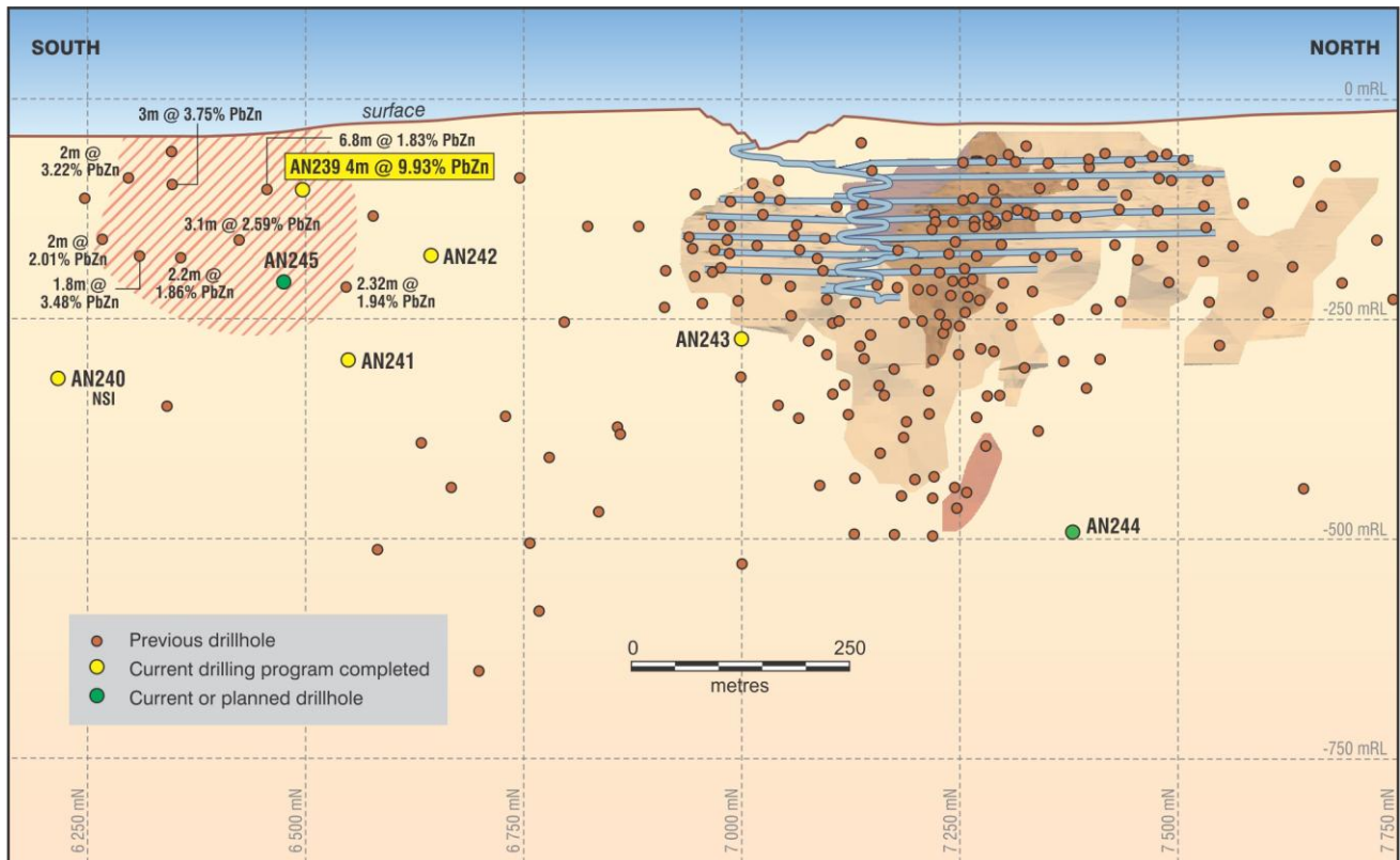
Figure 1: Section through the Angas Mine showing location of potential new shoot
